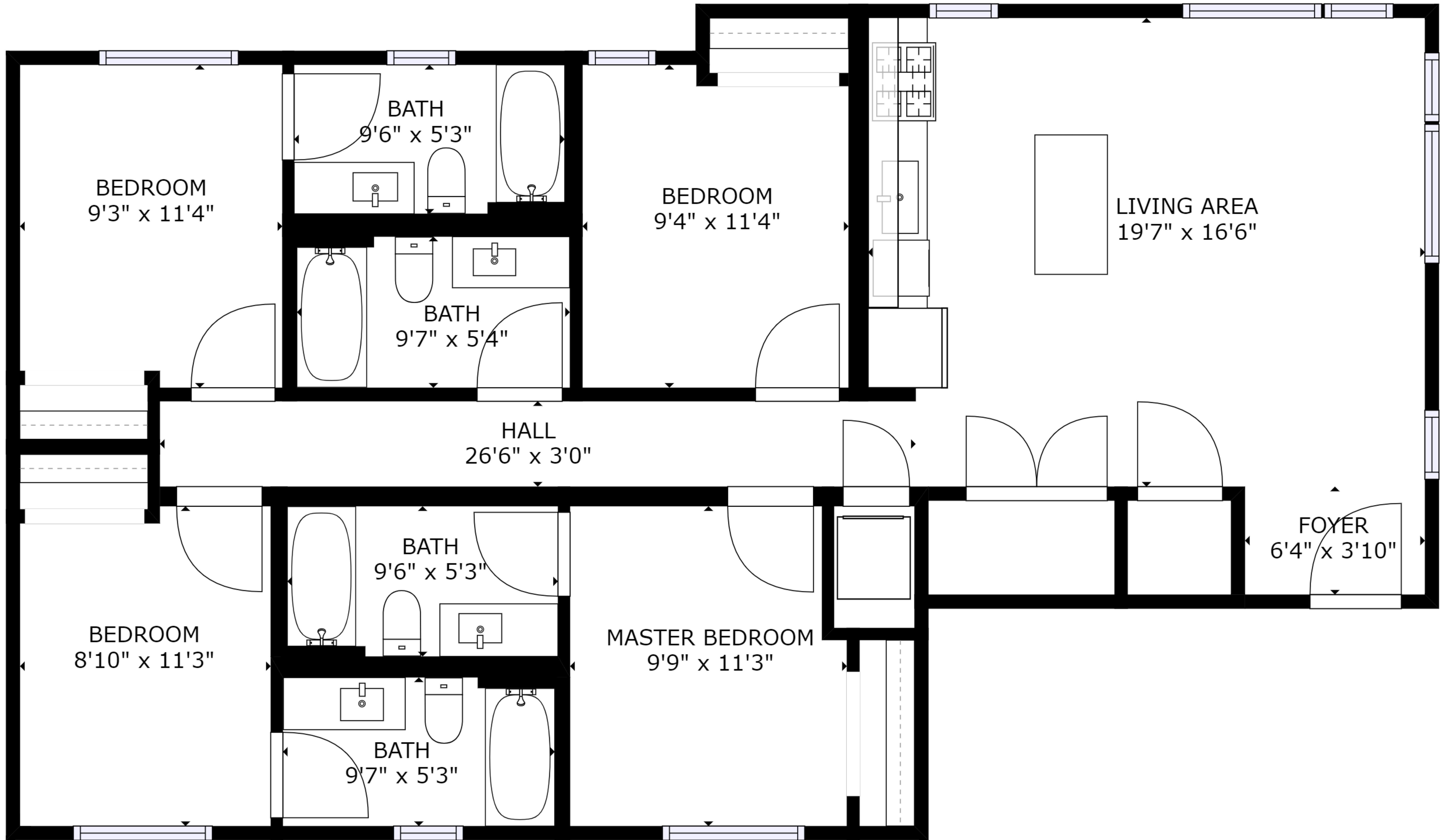
FLOOR 1
